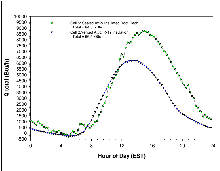
Figure 6. Estimated combined impact of duct heat gain, air leakage from the attic to conditioned space and ceiling heat flux on space cooling needs on an average summer day in a 2,000 ft 2 home.
