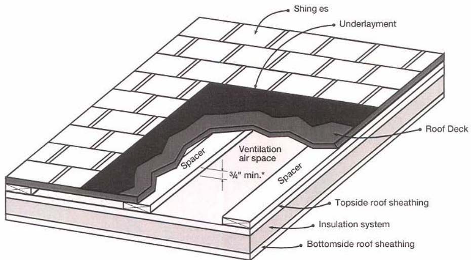
Figure C: Complete roofing assembly including spacers for ventilation
